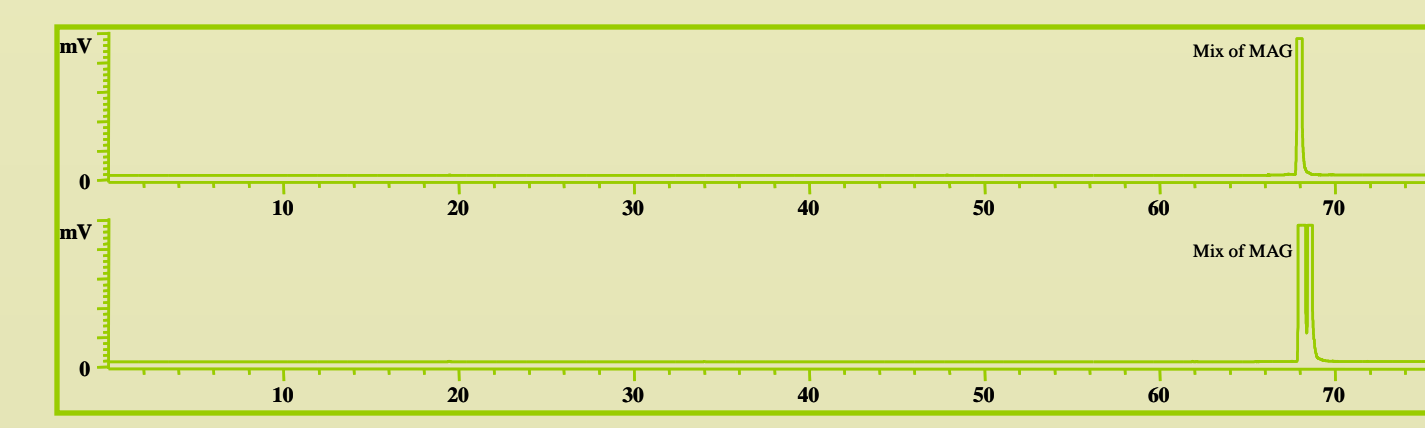
Fig. 8. Extracted ion chromatograms of starch lipids from maize flour.
