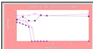
Figure 1. Effect of pH on the antimicrobial activity of chitosan upon S. aureus (-▲- pH 4 with chitosan; -△- pH 4 without chitosan; -■- pH 7 with chitosan; -□- pH 7 without chitosan). Other constant conditions: 0.2% NaCl, oleic and lactic acids present.
