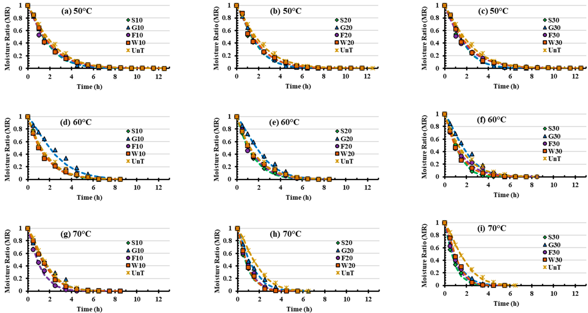
Figure 1. Drying kinetics of Satkara subjected to different US-OP conditions at (50, 60, and 70 °C). The dotted lines show the best model (Page) fit curves. S (sucrose), G (glucose), F (fructose), and W (distilled water) represent the four types of osmotic solution used. The numbers 10, 20, and 30 denote the duration (min) of the application of ultrasound. UT indicates the untreated sample.
