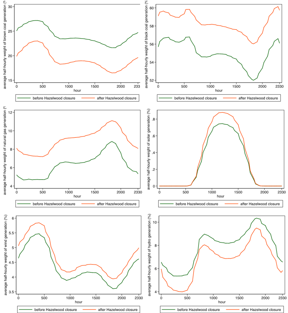
Figure 3: Weight of each type of electricity production, before and after closure, by half-hourly slots
