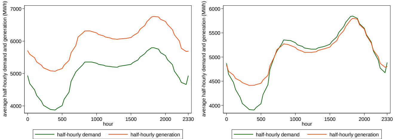
Figure 1: Electricity production and demand in the state of Victoria, before (left panel) and after (right panel) closure, by half-hourly slots
