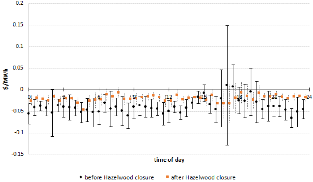
Figure 9: Indirect effect of the Hazelwood power plant closure: wind production
