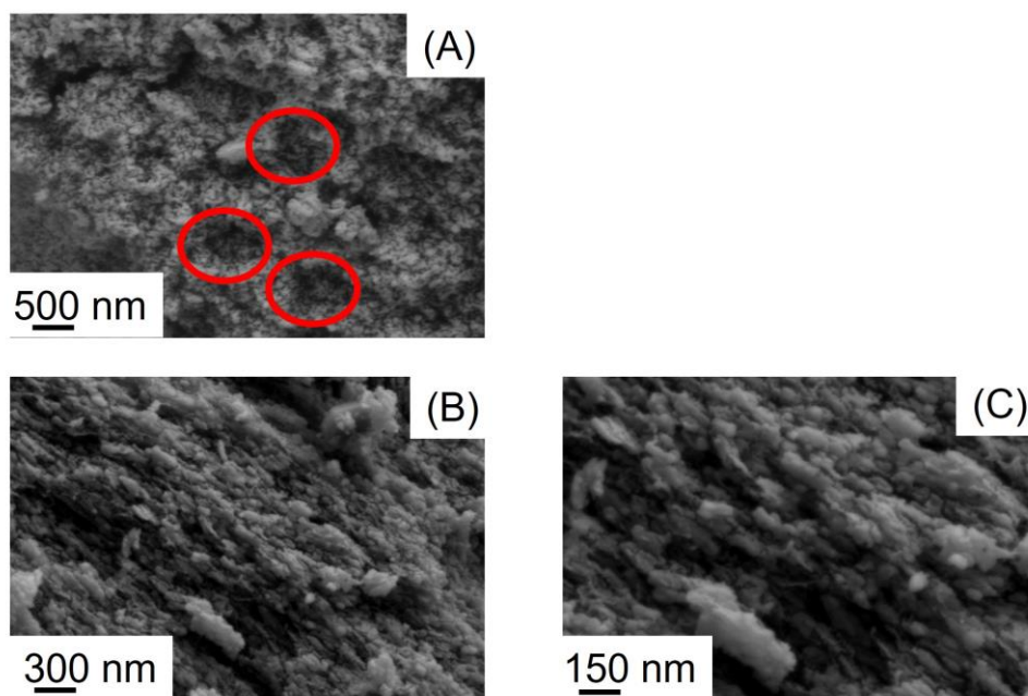
Figure 1. SEM micrographs of the TBC powder at various magnifications (A-C). Red circles in (A) indicate the formation of voids in the powder structure.
