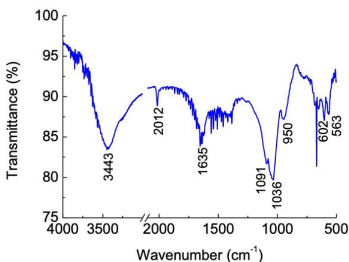
Figure 3. FTIR spectrum of TBC material.
