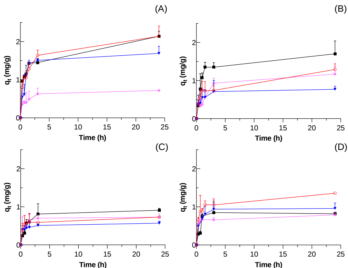
Figure 4. The adsorption capacity ( q_t ) of the TBC powder for each pharmaceutical, namely TRA and VNF when present alone (A and B, respectively), or as a mixture (C and D for TRA and VNF), in the different types of aqueous matrices. Adsorption assays were performed in four different aqueous matrices, namely in water (■), non-saline wastewater (○), saline wastewater with 7.5 g/L of sea salts (▼), and saline wastewater with 12 g/L of sea salts (*).
