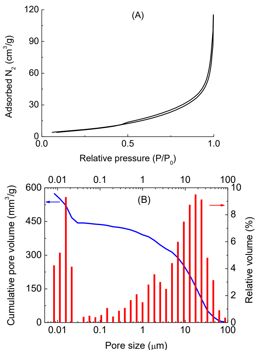
Figure 2. N 2 adsorption/desorption isotherm curve (A); the cumulative pore volume (blue line), and the histogram of the relative volume (red columns) as a function of the TBC powder pores size (B).
