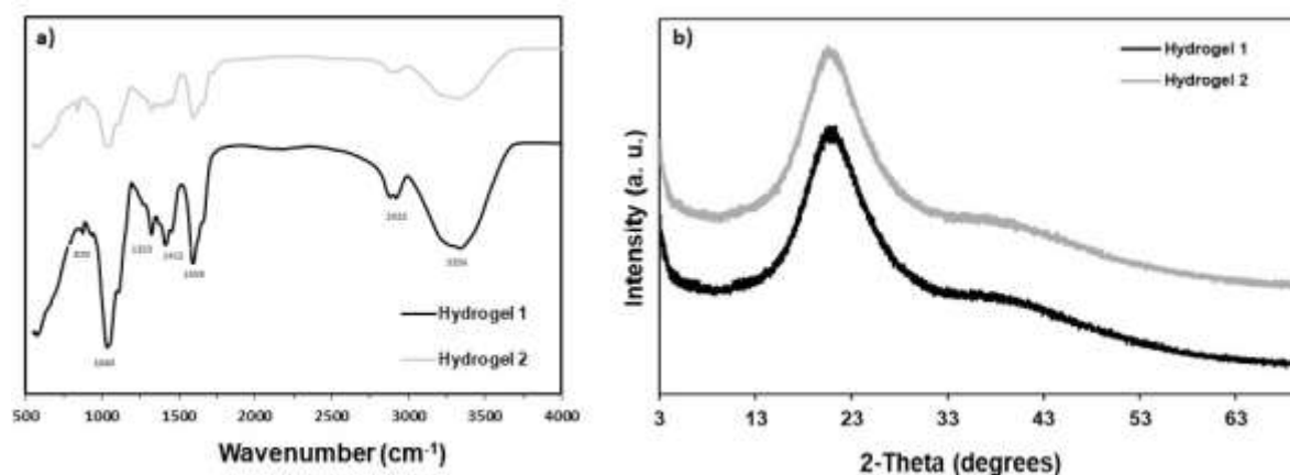
Figure 3. a) FTIR spectra of cellulose-based hydrogel prototype 1 (H1) and 2 (H2). b) Powder X-ray diffraction patterns of hydrogel prototypes H1 and H2. Note: H1 – cellulose-based hydrogel synthesized using natural cellulose fibers extracted from sugarcane bagasse; H2 cellulose-based hydrogel synthesized using commercial cellulose from Sigma-Aldrich.
