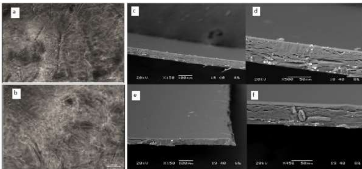
Figure 2. a) and b) Optical microscopy of H1 and H2, respectively. c) and d) Scanning electronic microscopy of H1 at x150 and at x450-500 magnification. e) and f) Scanning electronic microscopy of H2 at x150 and at x450-500 magnification. Note: H1 – cellulose-based hydrogel synthesized using natural cellulose fibers extracted from sugarcane bagasse; H2 – cellulose-based hydrogel synthesized using commercial cellulose from Sigma-Aldrich.
