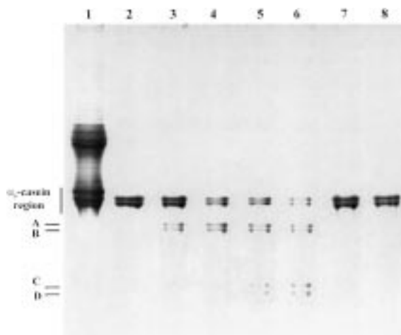
Fig. 3. Urea-PAGE electrophoregram of isolated \alpha_s -casein after hydrolysis by cardosin B for 1 min and 1, 3, 6 and 10 h (lanes 2–6). Lane 1 contains native ovine Na-caseinate, and lanes 7 and 8 contain ovine \alpha_s -casein after incubation for 1 min and 10 h, respectively, in the absence of enzyme, all included as controls.
