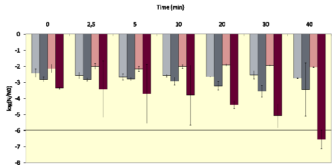
Figure 3. Inactivation of persistent and non-persistent L. monocytogenes strains, when exposed to the minimal inhibitory concentration of bleach.
