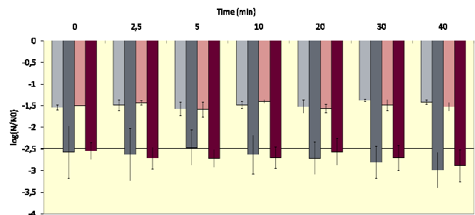
Figure 4. Inactivation of persistent and non-persistent L. monocytogenes strains, when exposed to the minimal inhibitory concentration of topax-66.
