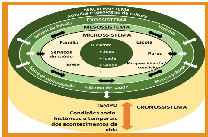
Ecological Theory
